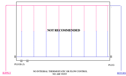
PANEL RADIATORS - ALTERNATE PIPING ARRANGEMENT 4
