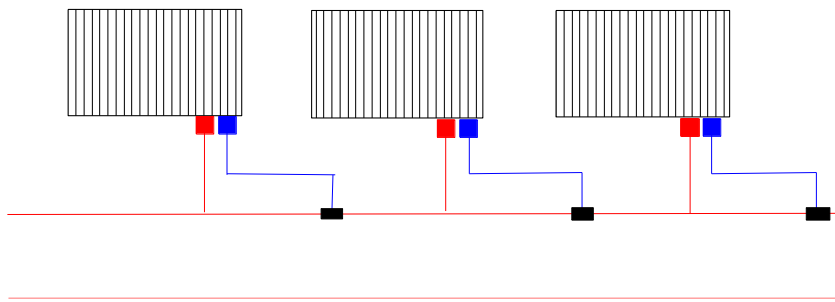
Monoflo (Diverter Tee)
